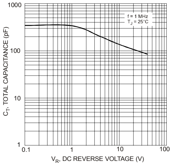
Fig. 5 Typical Capacitance
